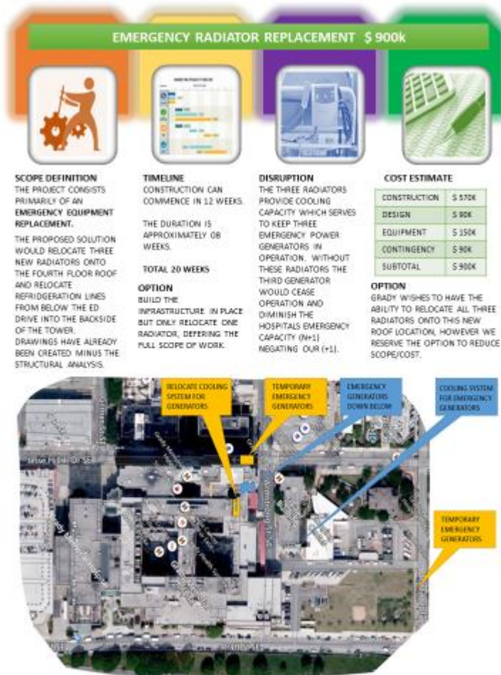
Figure #1 – Generator Cooling System Upgrade Concept
